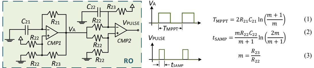
Fig. 1. Relaxation oscillator (RO) for the generation of V_{PULSE} .
