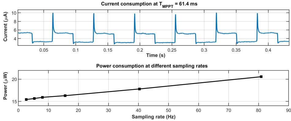
Fig. 2. Consumption of the RO. Top: current consumption at T_{\text{MPPT}} = 61.4 \text{ ms} . Bottom, average power consumption at different sampling rates.
