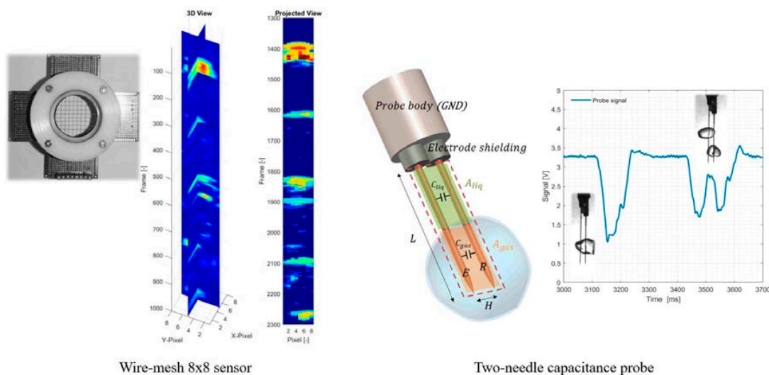
Fig 1. Example of a wire-mesh with 8 sensing lines and an example of slug bubble measured passing through the sensor (left). Detail of two-needle capacitive sensor and isolated bubbles measurement example signals (right).
