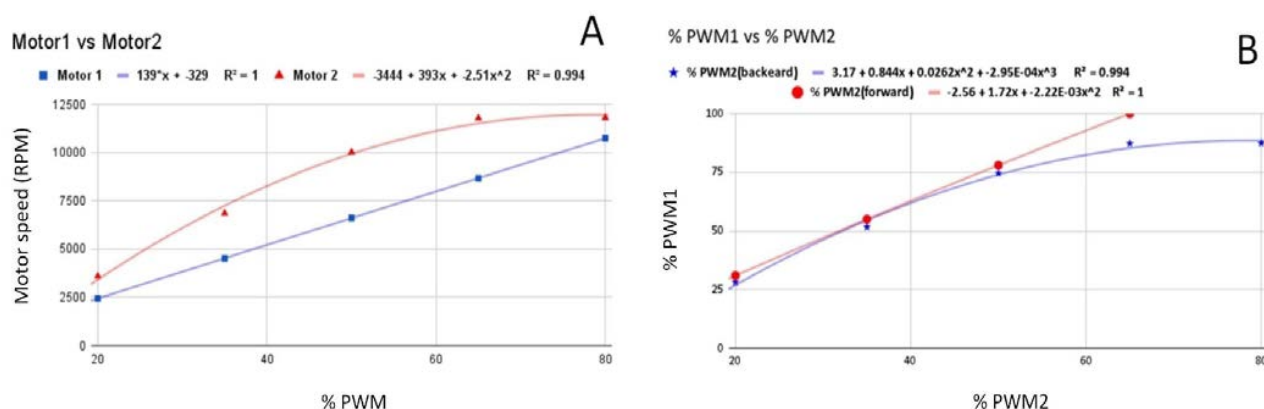
Figure 3 PWM pulses and speed of motors (A) and calibrated PWM2 based on PWM1 for the forward and backward movements (B).
