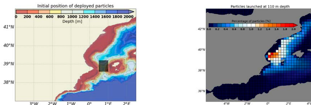
Fig 1. (Left) Map showing the initial location of deployed particles in the Ibiza Channel (black dots). Bottom depth is displayed in colour (unit in m). (Right) Annual mean of the percentage of particles according to their location 90 days before reaching the Ibiza Channel.
