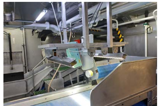
Fig 1. iObservers 2.0 installed on board R/V Miguel Oliver
