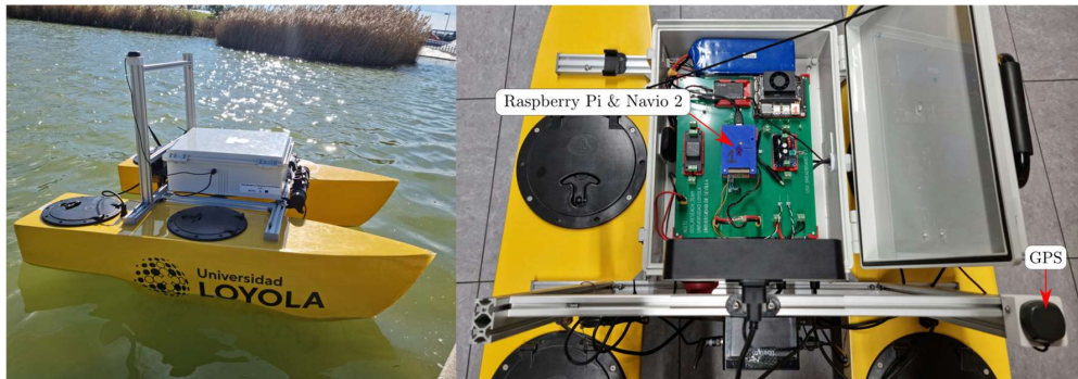
Fig 1. The Yellowfish ASV and the on-board sensors
