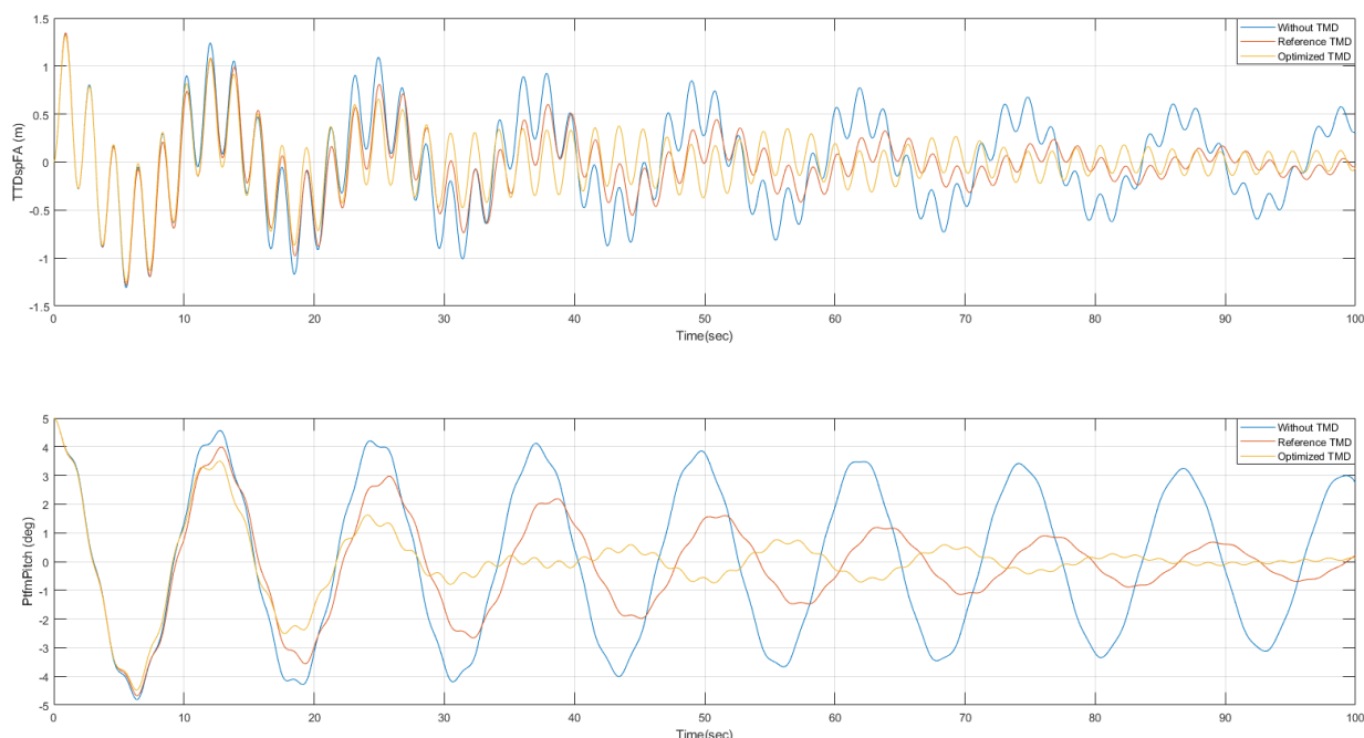
Fig 1. Example of the response of the WT without TMD and with the reference TMD y optimized TMD (platform pitch = 5^\circ ). Upper graph: fore-aft tower top displacement; bottom graph: platform pitch angle
