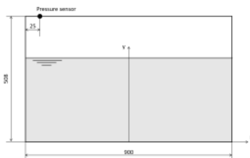
Fig. 1. Scheme of the experimental setup.
