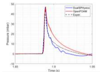
Fig. 2. Time series of pressure obtained with DualSPHysics (blue line), OpenFOAM (red line) and in the experimental tests (black dashed line).
