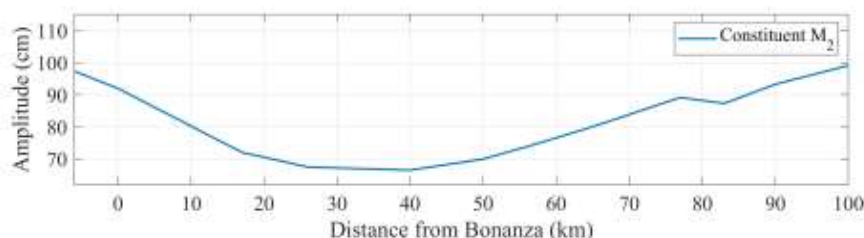
Fig 1. Profile of M_2 amplitude (cm) along the Guadalquivir Estuary.
