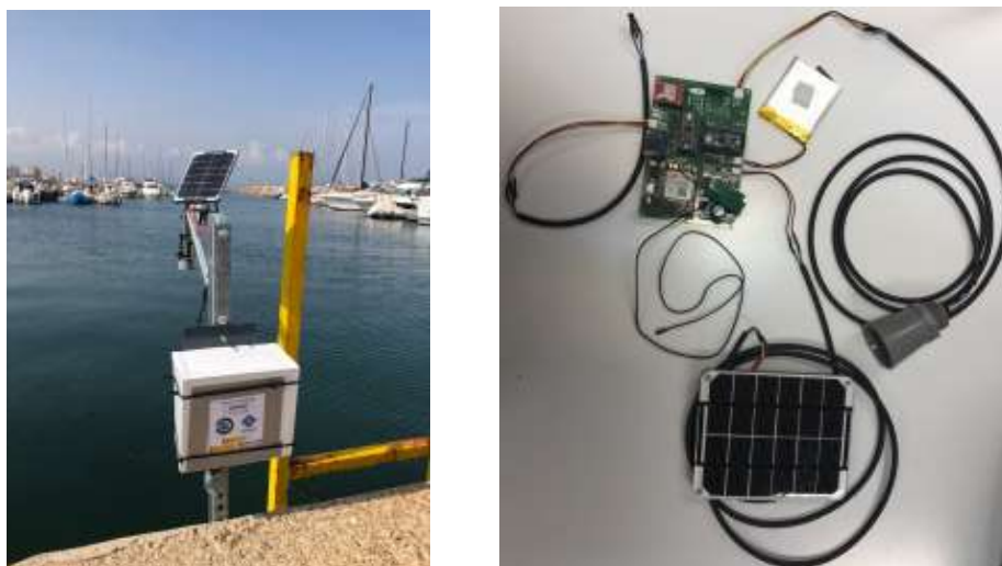
'Fig 1.' Low-Cost tide gauge (left) device and Arduino-based data logging circuit board (right).
