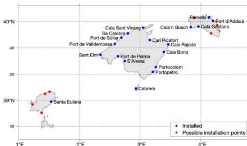
'Fig 2.' Tide gauge network locations operated by the VENOM project (blue) and future installation points (red).
