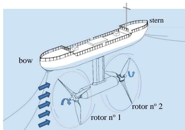
Fig. 1. Platform configuration
