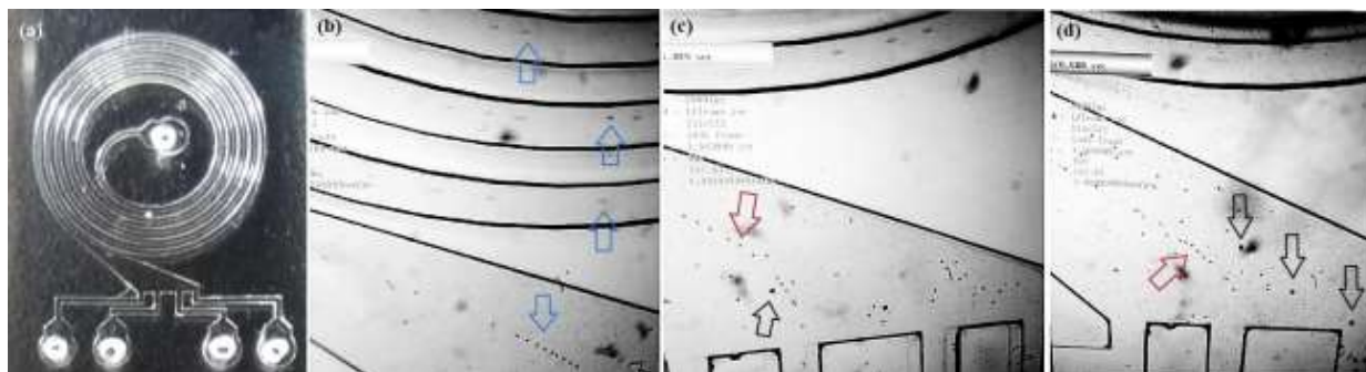
Fig 2. Experimental results: (a) PDMS spiral with four outlets; (b) Microparticles (blue arrows) being transported and focused at the microchannels for a flow rate of 1000 \mu\text{l}/\text{min} ; (c) 20 \mu\text{m} (red arrow) and 40 \mu\text{m} particles (black arrow) both exiting through the same outlet for a flow rate of 1000 \mu\text{l}/\text{min} ; (d) 20 \mu\text{m} (red arrow) and 40 \mu\text{m} particles (black arrow) with separated trajectories exiting through different outlet for a flow rate of 2000 \mu\text{l}/\text{min} .
