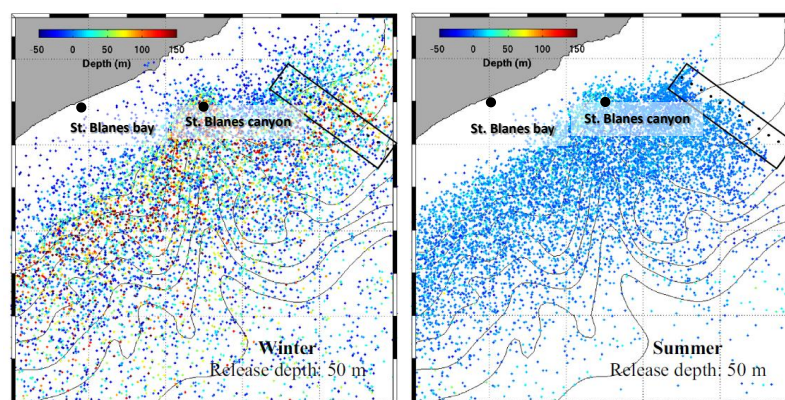
Fig. 3. Location of passive particles after 15-day tracking simulations around the OOCs observation stations (adapted with permission from Ahumada-Sempol et al. , 2015). Rectangles show initial particles release positions.
