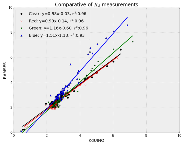
Fig. 1. Comparison of K_d results in four wavelength ranges (red, blue, green and visible) with two different instruments. They are highly linearly correlated.
