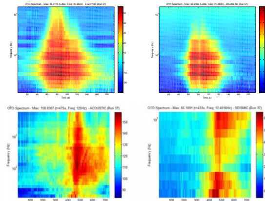
Fig. 6. Typical OTO of electric, (left-up), magnetic (right-up), acoustic (left-bottom) and seismic (right-bottom).
