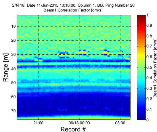
Fig. 7. Correlation factor indicates mooring line passing in front of beam 1 at around 30m. The cell will be contaminated, and a three beam solution omitting this beam should be selected.
