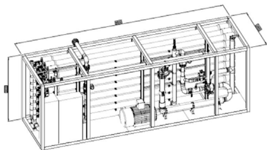
“Fig.4. Reverse Osmosis module”
