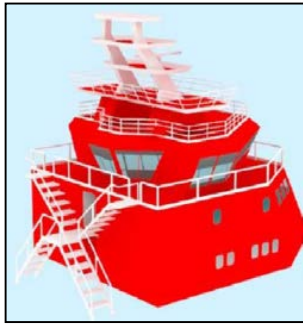
“Fig.2. 3D picture to the superstructure”
