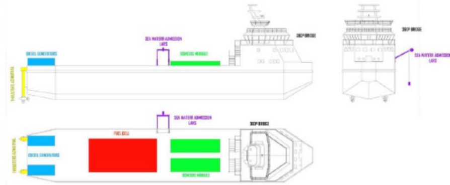
“Fig.1. General Arrangement”
