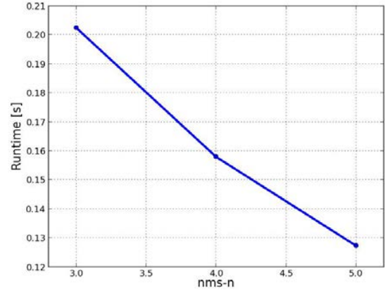
Fig. 2: Correlation between runtime and nms-n (Spearman coefficient of -0.72).
