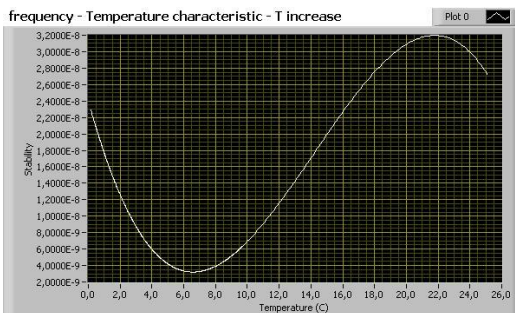
Fig. 5. f - T characteristic of the time base module.
