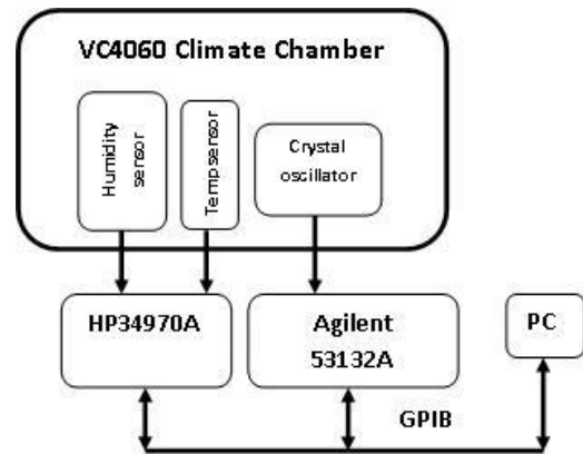
Fig. 2. Measurement system block diagram
