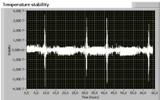
Fig. 4. Stability of the time base module
