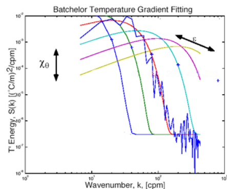
Figure 1 Batchelor temperature gradient fitting process to obtain the turbulent kinetic energy dissipation rate.
