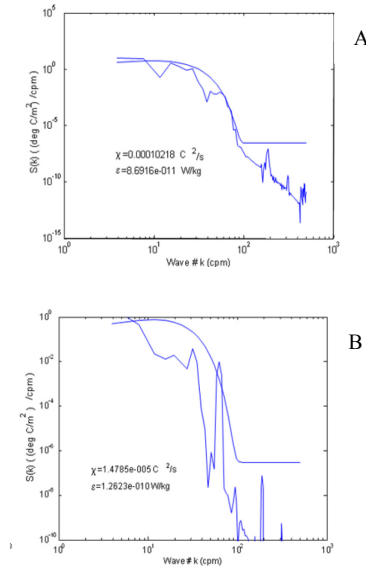
Figure 2 Batchelor temperature gradient fitting process to obtain epsilon. i.e: (a) represent well adjusted spectrum – (b) wrong adjuste.It is difficult to identify the error to reject the epsilon value.
