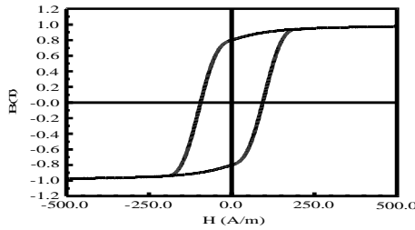
Fig.3. Hysteretic magnetic characteristic.
