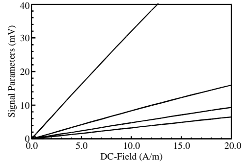
Fig.5. Output waveform parameters versus dc-field in the ferromagnetic cores.
