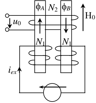
Fig.1. Fluxgate configuration used to measure an external dc-field.
